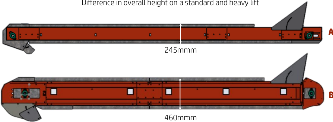
Difference in overall height on a standard and heavy lift
